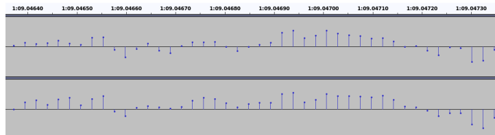
Figure 411: Plotting amplitude against time
